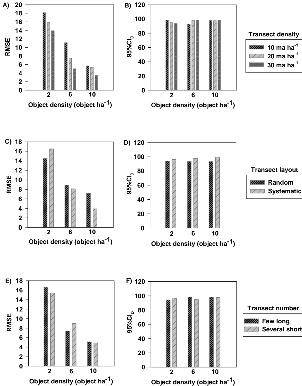
Fig. (2). Effect of total transect density (m ha -1 ), transect layout, and transect number on the accuracy of estimates of density obtained from the line transect method, and on the percentage of times 95% CI of estimated density contained the true density, for a random spatial distribution, and object densities ranging from 2 objects ha -1 to 10 objects ha -1 . The root mean squared error expressed as a percentage of D_T (RMSE) is plotted against (A) transect density (m ha -1 ), (C) transect layout, and (E) transect number for different object densities. The percentage of times 95% CI of \hat{D} contained D_T (95%CI b ) is plotted against (B) transect density (m ha -1 ), (D) transect layout, and (F) transect number, for different object densities.
