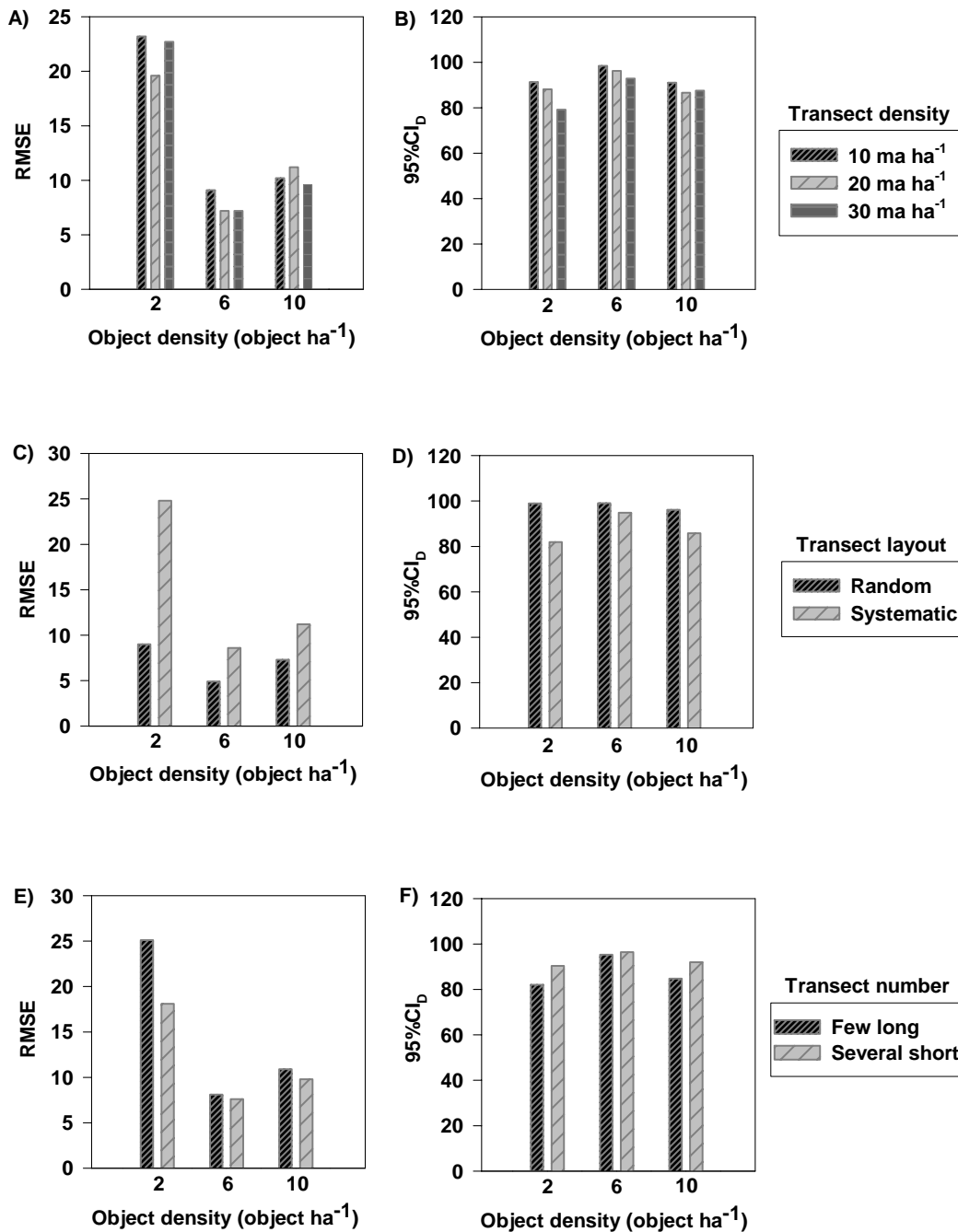
Fig. (3). Effect of total transect density ( m\ ha^{-1} ), transect layout, and transect number on accuracy of estimates of density obtained from the line transect method, and on the percentage of times 95% CI of estimated density contained the true density, for a uniform spatial distribution, and object densities ranging from 2 objects ha^{-1} to 10 objects ha^{-1} . The root mean squared error expressed as a percentage of D_T (RMSE) is plotted against (A) transect density ( m\ ha^{-1} ), (C) transect layout, and (E) transect number for different object densities. The percentage of times 95% CI of \hat{D} contained D_T ( 95\%CI_b ) is plotted against (B) transect density ( m\ ha^{-1} ), (D) transect layout, and (F) transect number, for different object densities.
