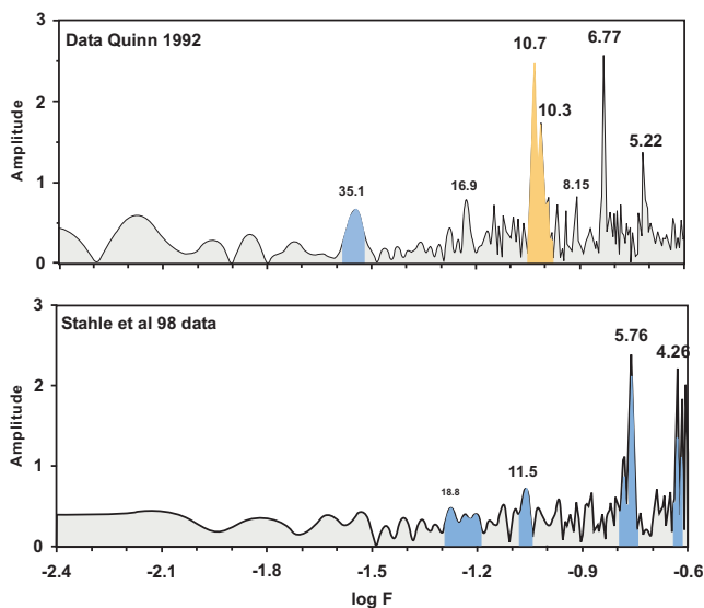
Fig. (7). Periodograms of ENSO-related reconstructions. Upper: ENSO history based on historical information. Lower: ENSO history inferred from tree-ring data. Sources: Quinn [53] and Stahle et al. [59]. Orange: here assumed sun-related. Blue: here assumed tide-related.
