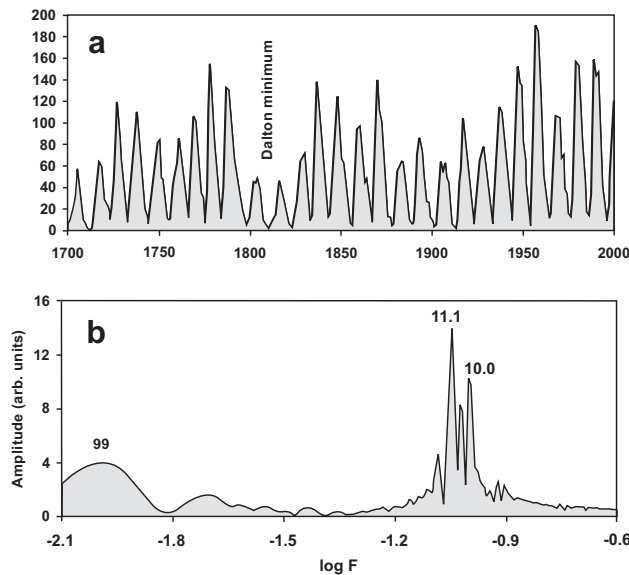
Fig. (2). Periodicity of the sunspot cycles between 1700 and 2000. Data source: Royal Astronomical Observatory of Belgium.
