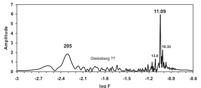
Fig. (4). Periodogram of aurora observations compiled by Schove [52], for the past 14 centuries.
