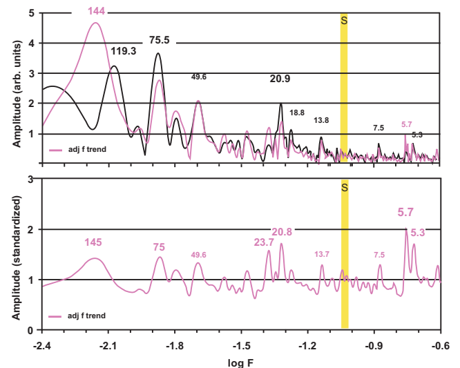
Fig. (5). Periodograms for the 500-year pine record near Flagstaff in Douglass [28] (Appendix, 1392-1906). Upper: black line, raw growth data; magenta, series adjusted for trend, including recalculation of local amplitudes of variation. Lower: additional recalculation of the adjusted periodogram in terms of mean and standard deviation within a gliding window of a factor of three. The mean is set at unity, the stdev. at 0.25.
