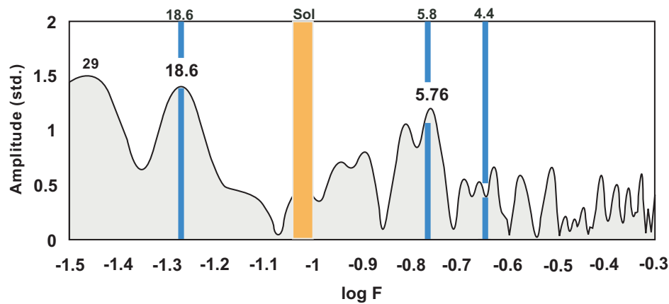
Fig. (8). Periodogram for the Pacific Decadal Oscillation in the 20 th century. Source of data: Mantua et al. [69], Zhang et al. [72], URL: http://www.atmos.washington.edu . The marked lines (18.6, 5.8, 4.4) are those expected for tidal activity.
