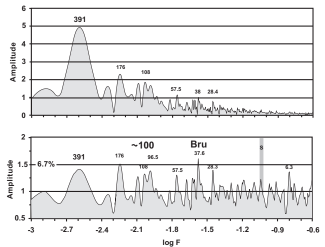
Fig. (6). Periodograms of the tree-ring series of Giant Sequoia, California, as given in Douglass [28], from AD 550. Upper: adjusted growth data, eliminating overall trend; lower: re-calculated periodogram, with standardized variation for a gliding window along log F of length factor-of-three. The mean is set at unity, and the standard deviation at 0.25. Two standard deviations (at 1.5) are equivalent to p=6.7\% . “Bru,” Brückner cycle.
