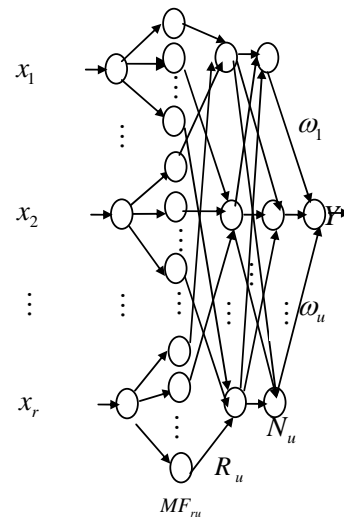
Fig. (1). Structure of dynamic fuzzy neural network.
