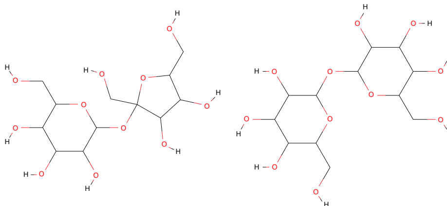
Fig. (1). Chemical structure of sucrose (left) and chemical structure of trehalose (right).
