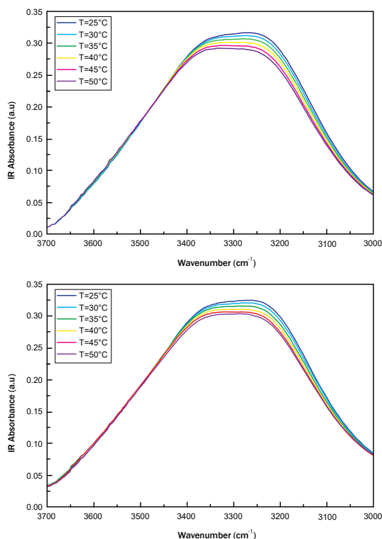
Fig. (2). a) OH-stretching region ( 3700 < \Delta\omega < 3000 \text{ cm}^{-1} spectral range) for different values of temperature, i.e. T=25°C, 30°C, 35°C, 40°C, 45°C and 50°C for sucrose water mixture and b) OH-stretching region ( 3700 < \Delta\omega < 3000 \text{ cm}^{-1} spectral range) for different values of temperature, i.e. T=25°C, 30°C, 35°C, 40°C, 45°C and 50°C for trehalose water mixture.
