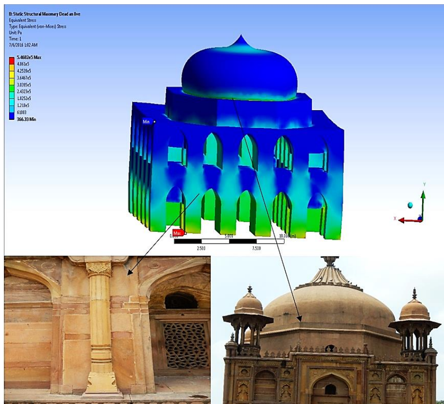
Fig. (6). Stress pattern and its location in real structure due to static loading.
