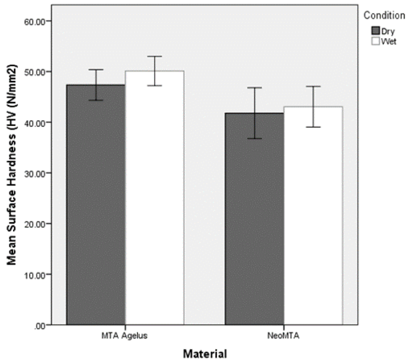
Fig. (4). Microhardness at 4 mm from the proposed apex (Error bars 95% CI).
