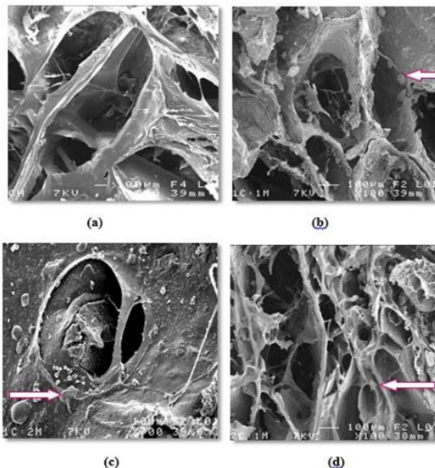
Fig. (9). SE micrograph for the internal surface of C, 1C:1M, 1C:2M, and 2C:1M scaffolds with \times 100 magnification [a-d]. The arrows show the HA precipitation.
