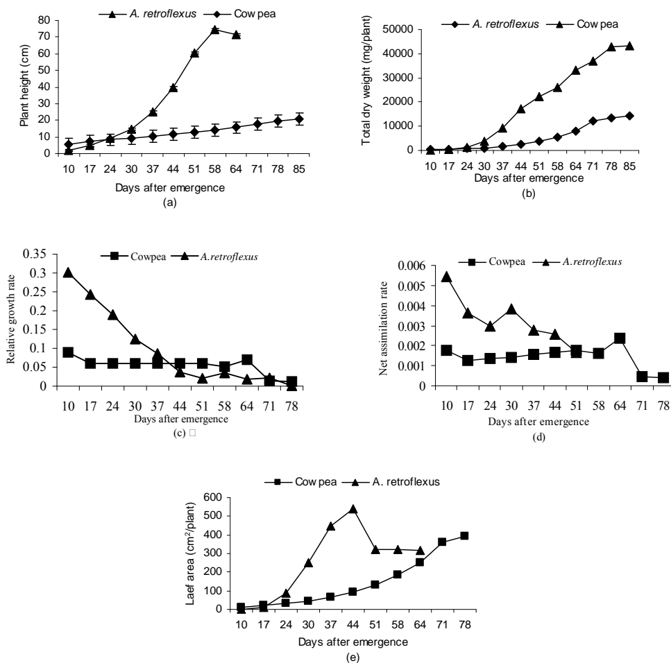
Fig. (3). Comparative a) plant height, b) total dry weight, c) relative growth rate, d) net assimilation rate and e) leaf area of cowpea and A. retroflexus grown in pure stands for different periods. Error bars indicate SE of the means.
