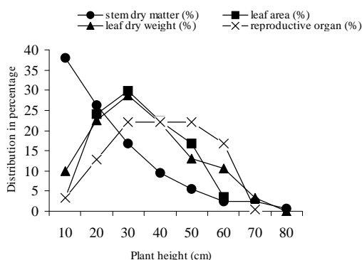
Fig. (4). Distribution percentages of stem dry weight, leaf area, leaf dry weight and reproductive organ of A. retroflexus in relation to its height.
