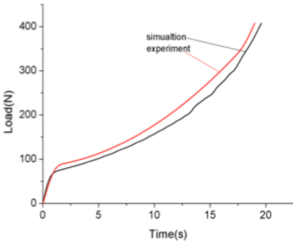
Fig. (7). Load variation data obtained by experiment and simulation at 560 °C.
