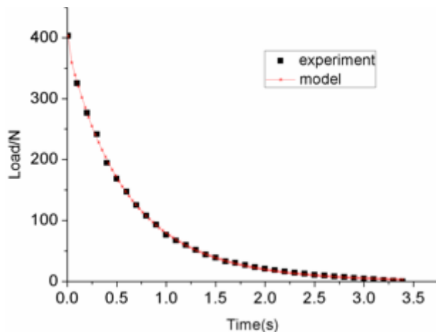
Fig. (4). Comparison of Load Relaxation between Experiment Data and Fitting Data Using a 4-pair General Maxwell Model at 560°C.
