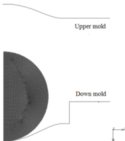
Fig. (8). FEM model of lens molding.
