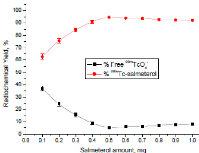
Fig. (2). Radiochemical yield of ^{99m}\text{Tc} -salmeterol xinafoate as a function of salmeterol xinafoate amount. Reaction conditions: Xmg salmeterol xinafoate, 10 mg of \text{NaBH}_4 , pH 9, 1 mL (~400 MBq) of ^{99m}\text{TcO}_4^- solution, room temperature, 30 min.
