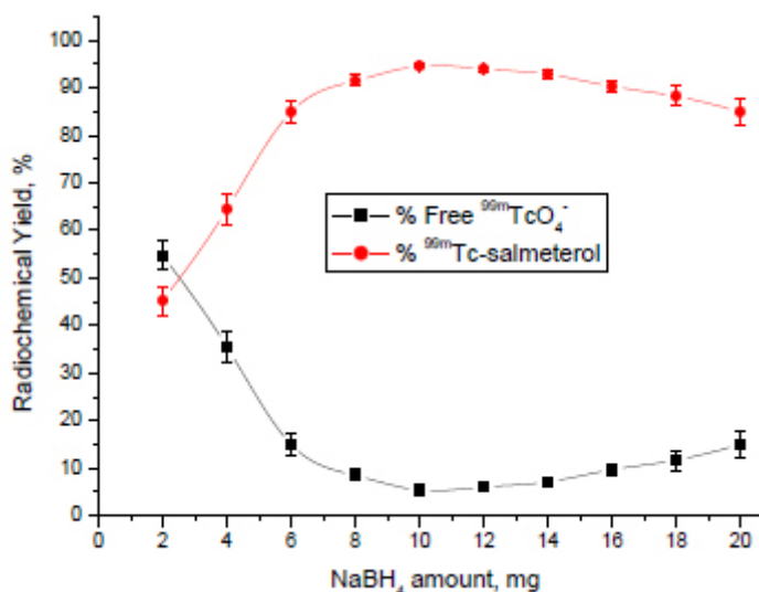
Fig. (3). Radiochemical yield of ^{99m}\text{Tc} -salmeterol xinafoate as a function of \text{NaBH}_4 amount. Reaction conditions: 0.5 mg salmeterol xinafoate, X mg of \text{NaBH}_4 , pH 9, 1 mL (~400 MBq) of ^{99m}\text{TcO}_4^- solution, room temperature, 30 min.
