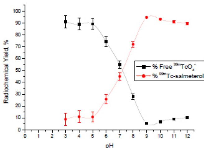
Fig. (4). Radiochemical yield of ^{99m}\text{Tc} -salmeterol xinafoate as a function of pH amount. Reaction conditions: 0.5 mg salmeterol xinafoate, 10 mg of \text{NaBH}_4 , pH = X, 1 mL (~400 MBq) of ^{99m}\text{TcO}_4^- solution, room temperature, 30 min.
