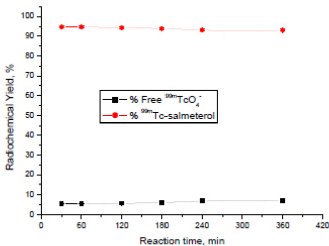
Fig. (6). Radiochemical yield of ^{99m}\text{Tc} -salmeterol as a function of the reaction time. Reaction conditions: 0.5 mg salmeterol, 10 mg of \text{NaBH}_4 , pH = 9, 1 mL (~400 MBq) of ^{99m}\text{TcO}_4^- solution, room temperature, X min reaction time.
