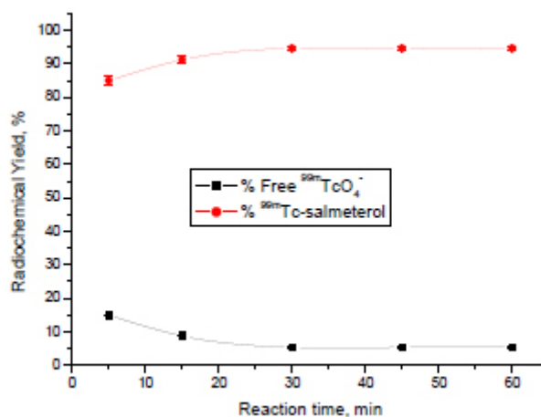
Fig. (5). Radiochemical yield of ^{99m}\text{Tc} -salmeterol xinafoate as a function of the reaction time. Reaction conditions: 0.5 mg salmeterol, 10 mg of \text{NaBH}_4 , pH = 9, 1 mL (~400 MBq) of ^{99m}\text{TcO}_4^- solution, room temperature, X min reaction time.
