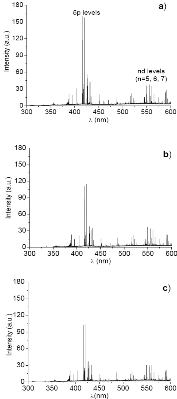
Fig. (3). Spectra of an Ar/He discharge recorded in the 300-600 nm region for different He concentration: 0 % (a), 10 % (b) and 30 % (c).
