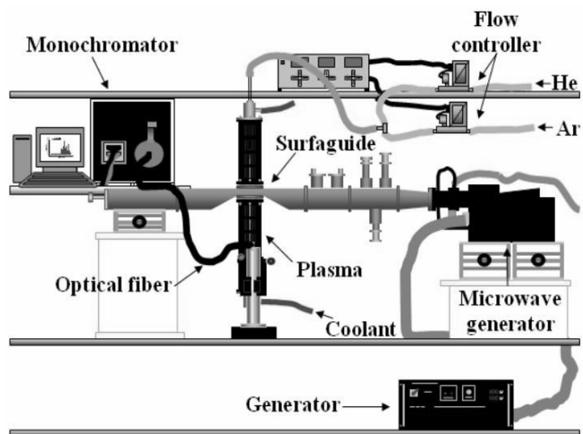
Fig. (1). Experimental device.
