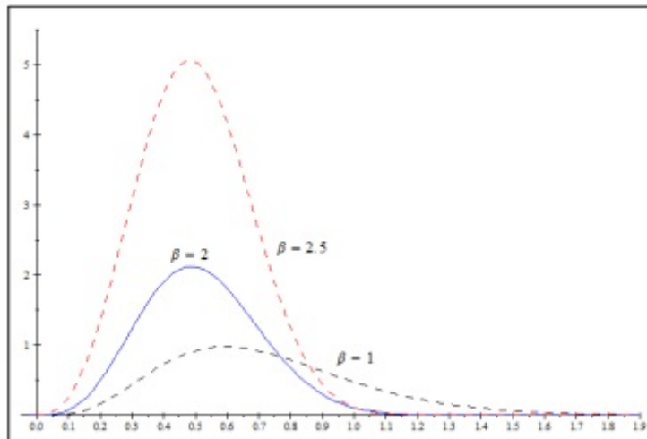
Fig. (4). Graph of the pdf (3) for s=6, r=8, alpha=4 and for various values of beta (for beta=2 this is model 4).
