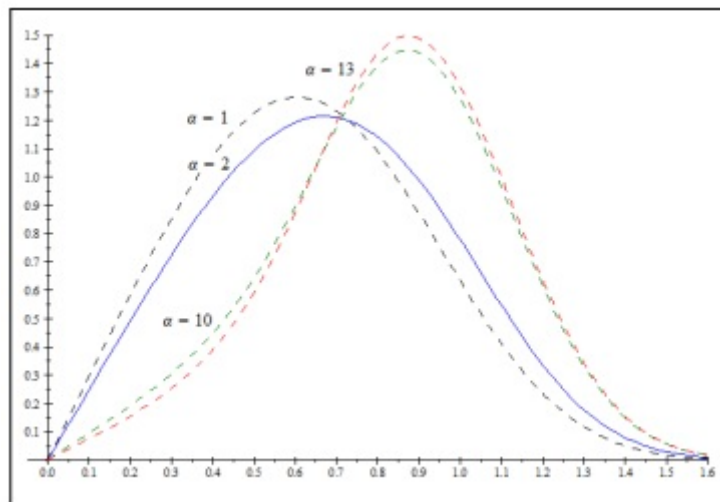
Fig. (2). Graph of the pdf (3) for s=5, r=2, \beta=3 and for various values of \alpha (for \alpha=2 this is model 2).
