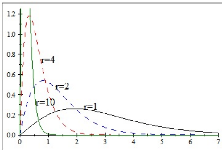
Fig. (3). Graph of the pdf (3) for s=3, \alpha=2, \beta=1 and for various values of r (for r=10 this is model 3).
