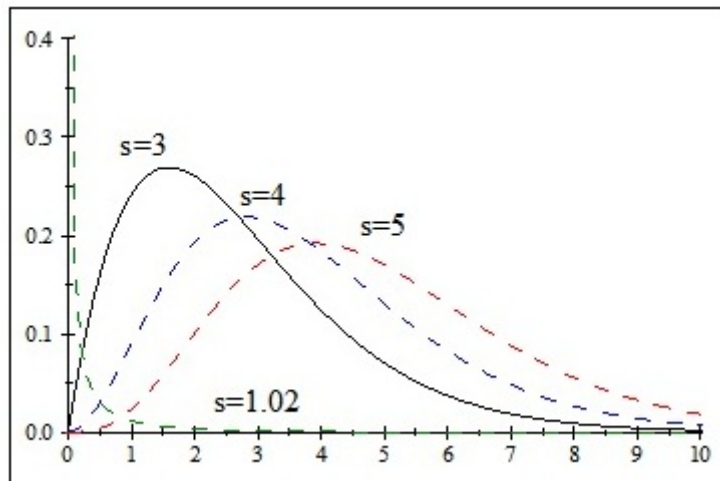
Fig. (1). Graph of the pdf (3) for r=\alpha=\beta=1 and for various values of s (for s=3 this is model 1).
