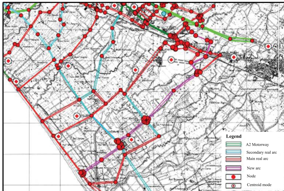
Fig. (9). Road graph intervention scenario.
