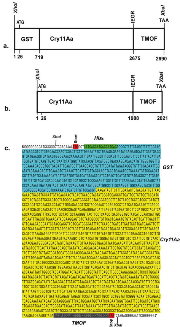
Fig. (2). Genomic organization of cry11Aa-tmf synthetic gene. a. gst-cry11Aa-tmfA (2,690 nt) genetic map with restriction enzymes cleavage sites for cloning, the ATG start signal, the IEGR trypsin cleavage site and the TAA stop signal. b. cry11Aa-tmfA (2,021 nt) genetic map with restriction enzymes cleavage sites for cloning, IEGR trypsin cleavage site and start (ATG) and stop (TAA) signals. c. gst-cry11Aa-tmf optimized synthetic gene sequence: His 6 -gst (green-blue), cry11Aa (yellow) and tmfA (grey), with the stop and start signals (red).
