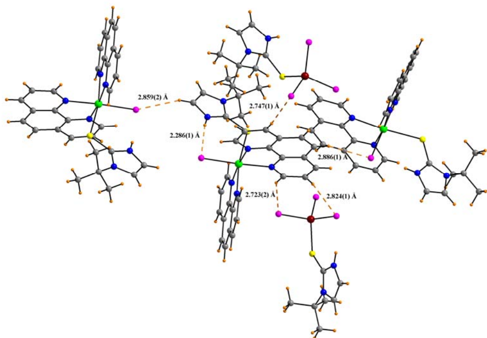
Fig. (S4). Intermolecular C-H...Cl interactions (pink dotted) shown by one cation molecule with anion molecules in complex 4.
