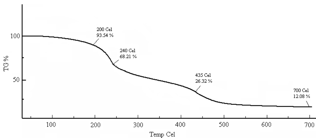
Fig. (S9). TGA spectra for complex 2.
