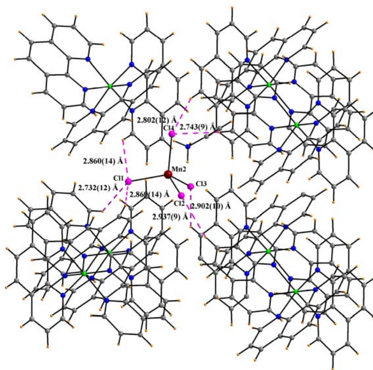
Fig. (S1). Intermolecular C-H...Cl interactions (pink dotted) shown by one anion molecule with cation molecules in complex 1.
