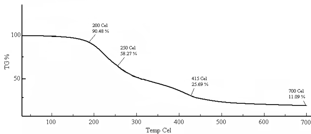
Fig. (S10). TGA spectra for complex 4.
