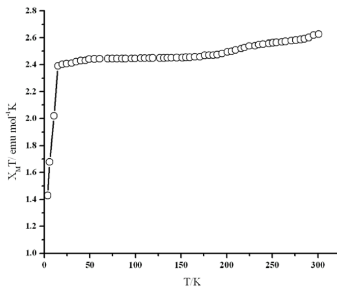
Fig. (S7). Temperature dependence of the \chi_M T product for complex 4.
