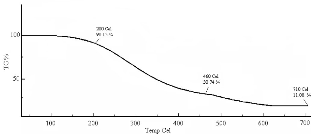
Fig. (S8). TGA spectra for complex 1.
