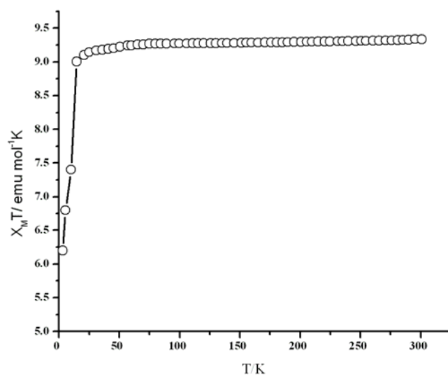
Fig. (S6). Temperature dependence of the \chi_M T product for complex 2.
